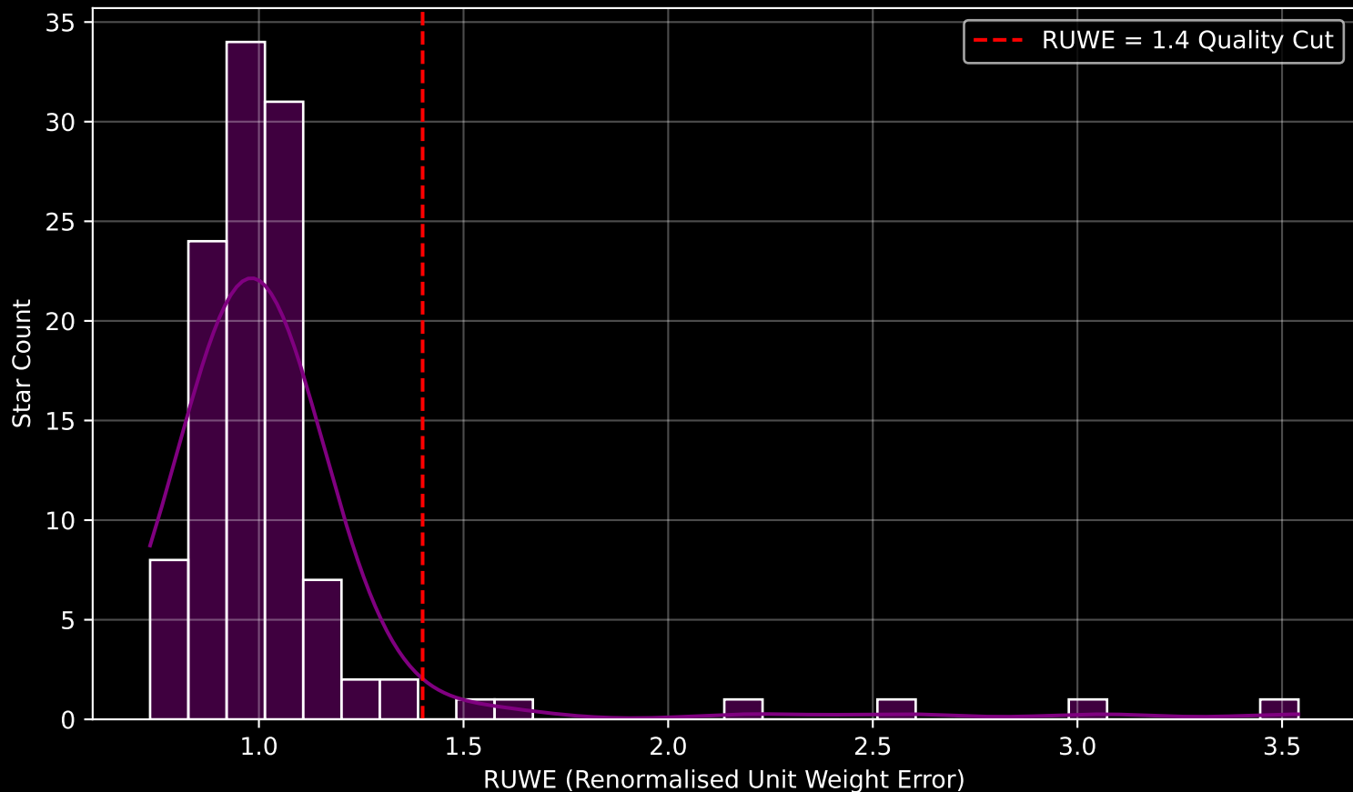
GAPOGEE DR17 Field [002+06] RUWE Distribution (n= 114)
