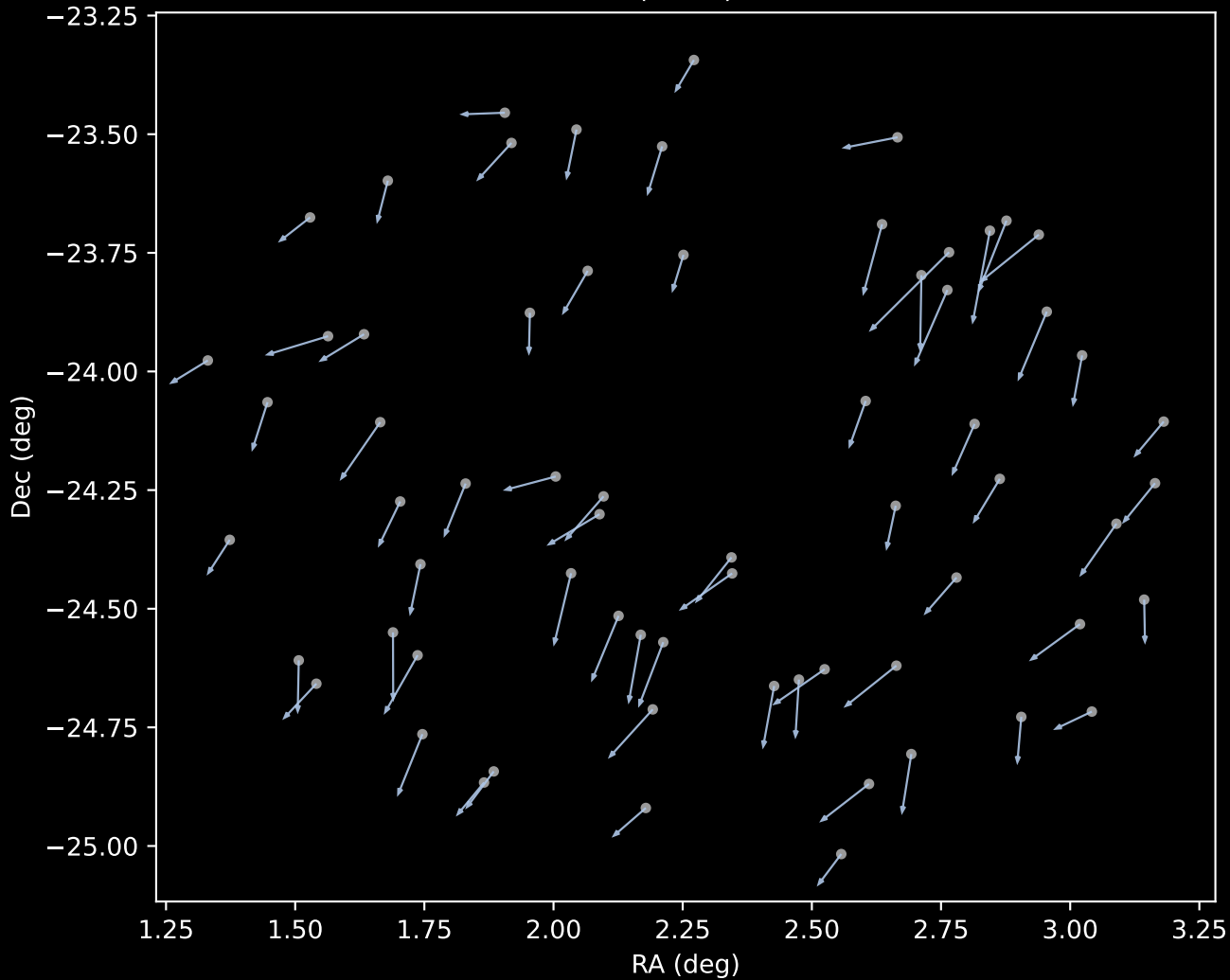
APOGEE DR17 Cluster 1 Proper Motion Vectors (n=66)
