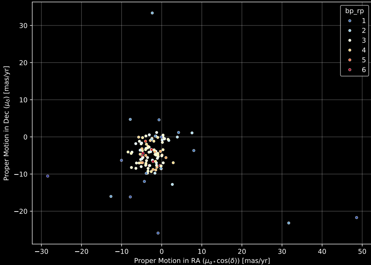
APOGEE DR17 Field: [002+06] Proper Motion Diagram (n= 115)
