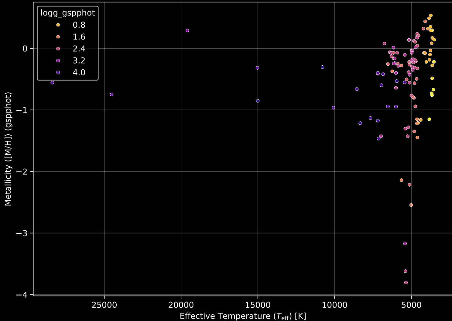
APOGEE DR17 Field: [002+06] Stellar Population Parameters (n= 115)
