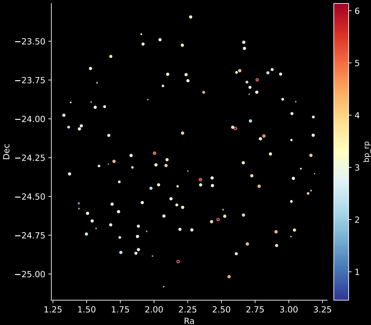
APOGEE DR17 Field: [002+06] Stars: 115
