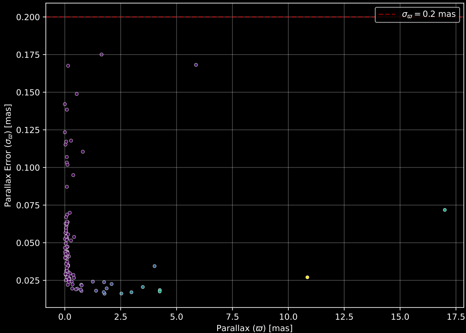
APOGEE DR17 Field: [002+06] Parallax Quality (n= 115)
