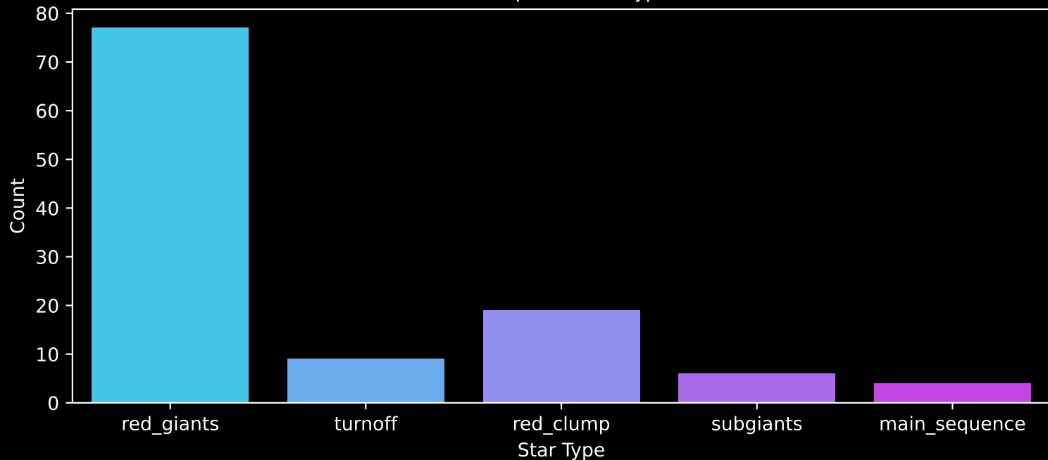
APOGEE DR17 Field: [002+06] Count plot of Star Type
