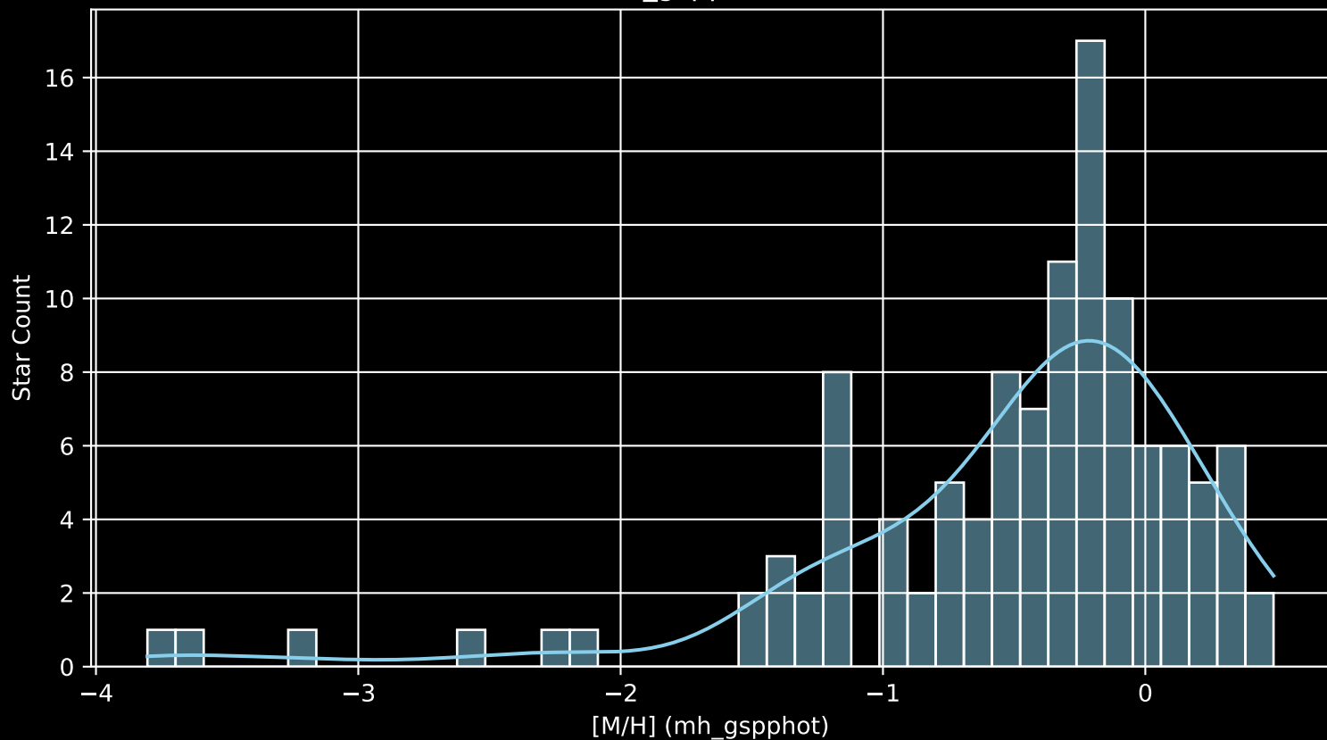
APOGEE DR17 Field: [002+06 [M/H] (mh_gspphot) (n= 114)
